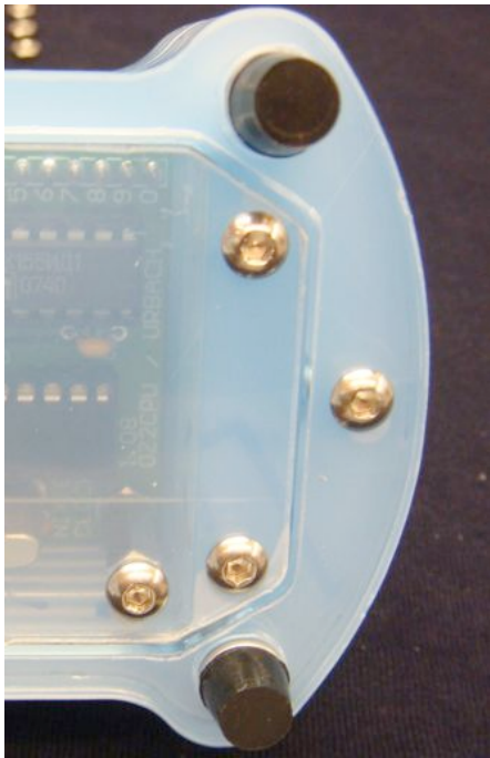
Figure 11 - case bottom screws fit in 3 mm thread
